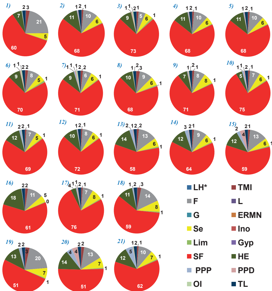
Figure 2. Main energy expenditure (%) on the charts and total energy consumed (GJ ha -1 ) (a), total energy produced (GJ ha -1 ) (b) in the agricultural stage of second crop maize in the following caption. 1) FAEG-GO, a=12.8 and b=99.7; 2) Rio Verde-GO, a=11.4 and b=77.1; 3) Montividiu-GO, a=11.8 and b=135.1; 4) Montividiu-GO, a=13.0 and b=161.4; 5) Rio Verde-GO, a=13.0 and b=134.2; 6) Montividiu-GO, a=12.3 and b=113.3; 7) Montividiu-GO, a=10.1 and b=112.4; 8) Montividiu-GO, a=10.1 and b=90.7; 9) Rio Verde-GO, a=8.3 and b=136.0; 10) Montividiu-GO, a=10.1 and b=154.1; 11) Montividiu-GO, a=10.6 and b=136.0; 12) Sorriso-MT, a=11.4 and b=81.6; 13) Campo Novo do Parecis-MT, a=10.2 and b=90.7; 14) Campo Verde-MT, a=10.5 and b=90.7; 15) Primavera do Leste-MT, a=11.1 and b=90.7; 16) Passo Fundo-RS, a=13.4 and b=72.5; 17) Ubiratã-PR, a=8.3 and b=86.1; 18) Campo Mourão-PR, a=8.2 and b=68.0; 19) Londrina-PR, a=8.8 and b=78.6; 20) Unaí-MG, a=8.7 and b=86.1; 21) Chapadão do Sul-MS, a=9.9 and b=99.7. * Human labor (HL), Tractors, machinery and agricultural implements (TMI), Fuels (F), Lubricants (L), Grease (G), Energy used in the repair of tractors, machinery, and agricultural implements (ERMN), Seeds (Se), Inoculants (Ino), Limestone (Lim), Gypsum (Gyp), Industrial fertilizers (SF), Herbicides (HE), Plant protection products for the control of pests (PPP), Plant protection products for the control of diseases (PPD), Other inputs (OI), Transportation of machinery, implements, and inputs to the field (TL). Labels of slices <1% were not shown in the pie charts.
