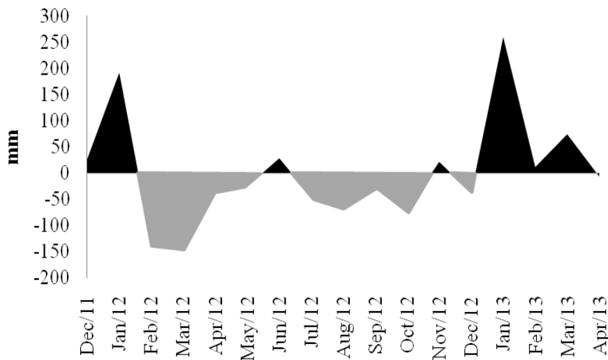
Figure 2. Extract of the monthly water balance of December 2011 to April 2013, according to Thornthwaite & Mather (1955) - Source: Site Data Bank of the National Institute of Meteorology (INMET).
