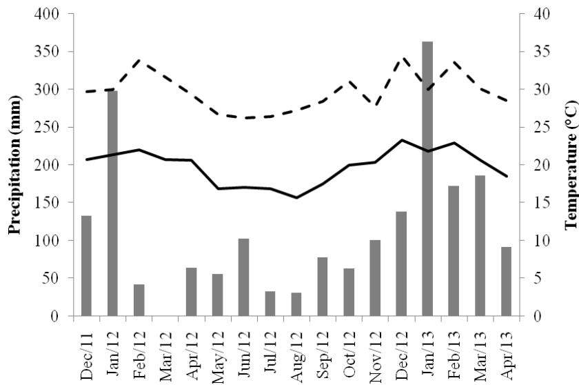
Figure 1. Precipitation (mm), temperatures maximum – °C (---) and minimum – °C (-) December of de 2011 of April of 2013 of the experimental area.
