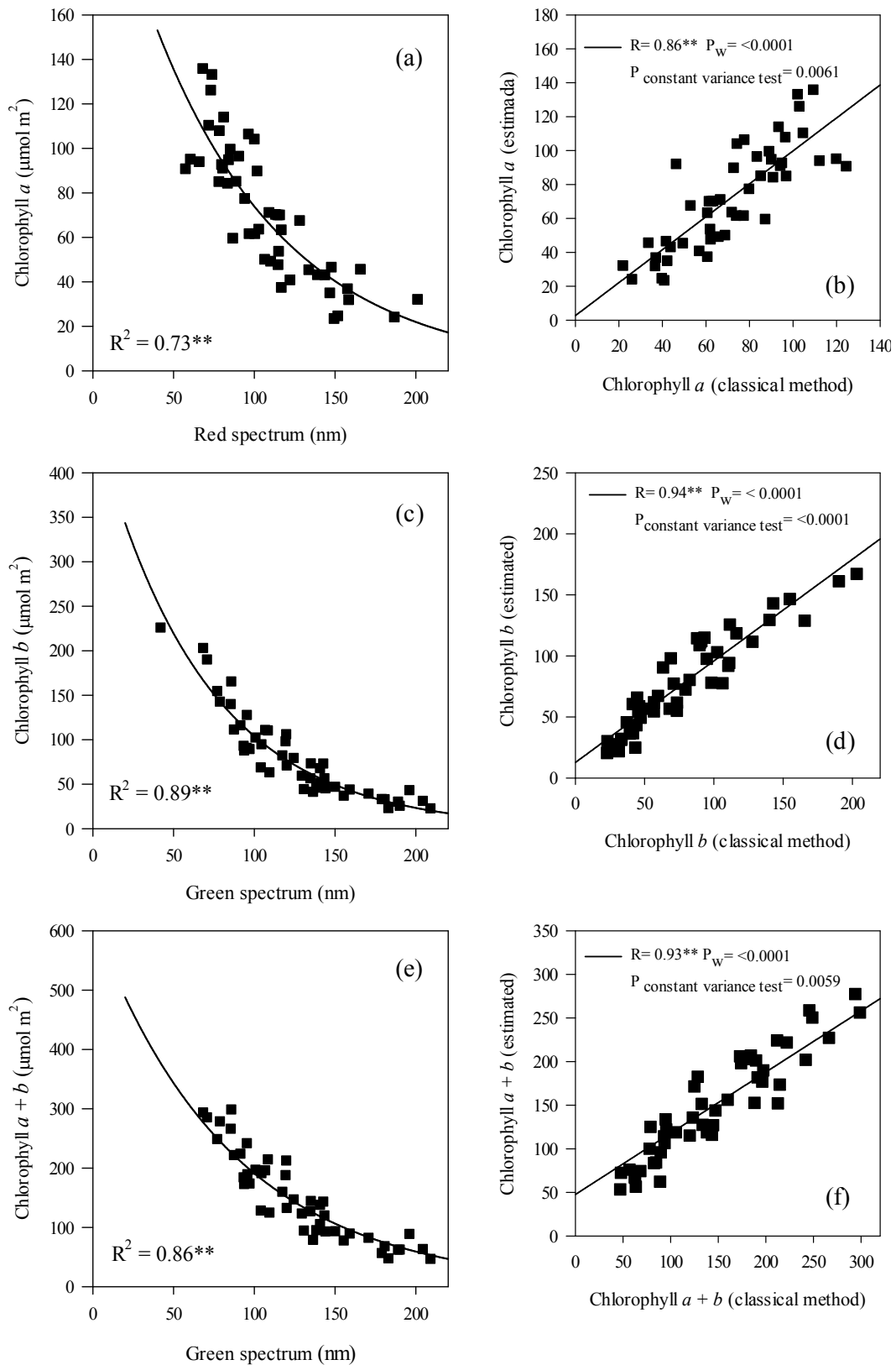
Figure 1. Adjusted equations and analysis of residuals between red and green spectral values with the content chlorophyll a (a, b), b (c, d) and a + b (e, f) in E. dunnii leaves.
